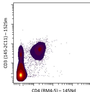
Mouse splenocytes stained with 152Sm anti-CD3 (145-2C11) and 145Nd anti-CD4 (RM4-5). Viable cells are displayed in the analysis.
